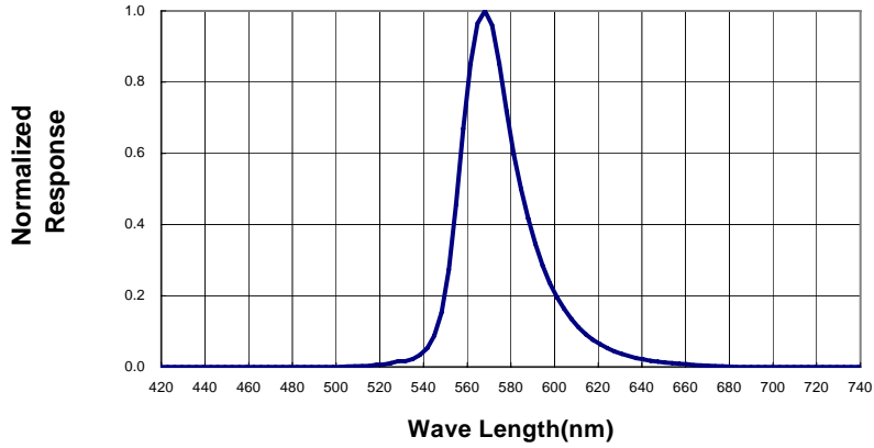
Spectral Radiance (Peak @ 568nm)
