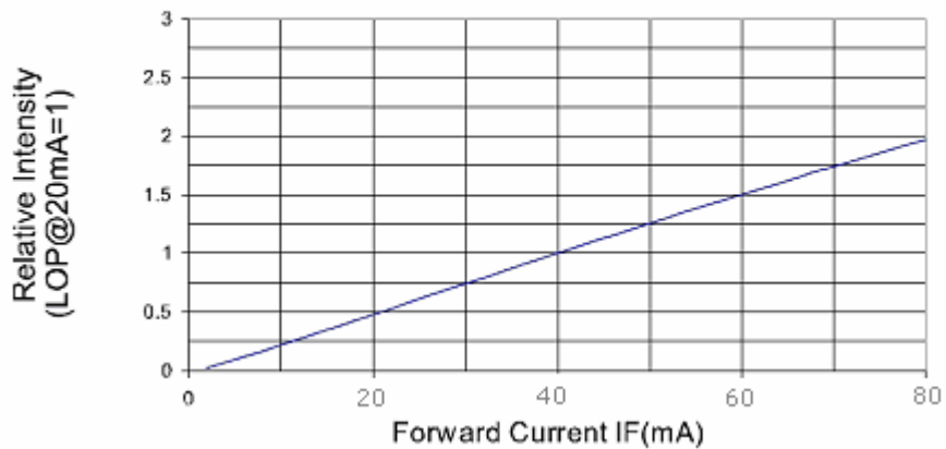
Relative Luminous Intensity vs Forward Current
